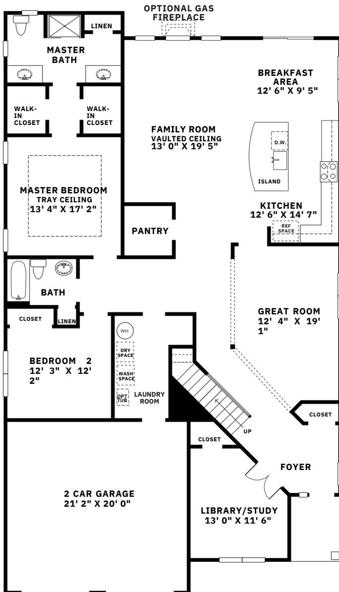
First Floor
