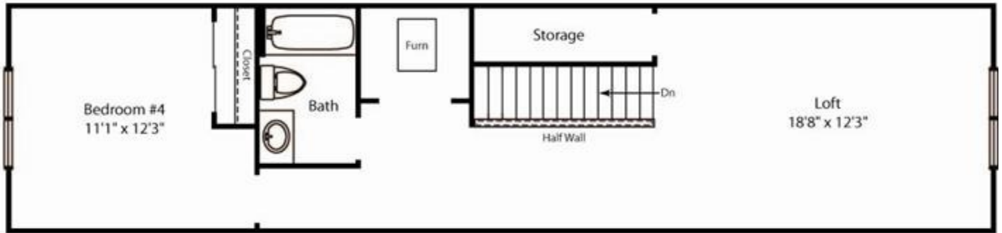
Raphael Optional Loft & 4th Bedroom
