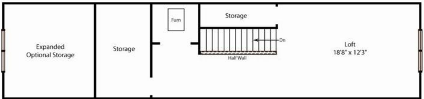
Raphael Second Floor Plan
