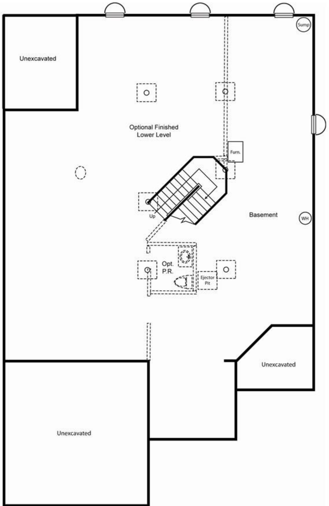
Matisse Optional Basement Plan (with Finished Lower Level Option)
