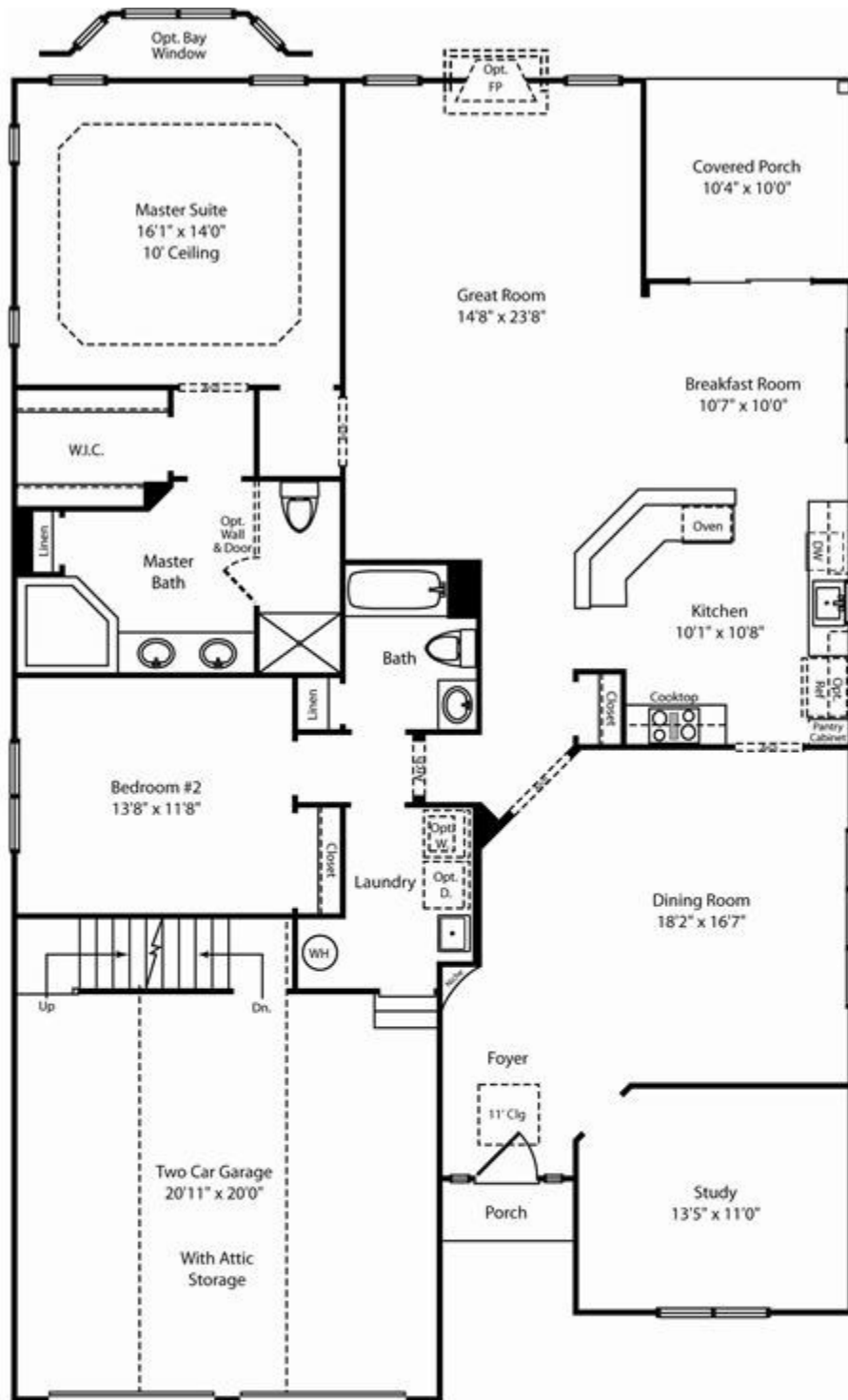
Geneva First Floor Plan
