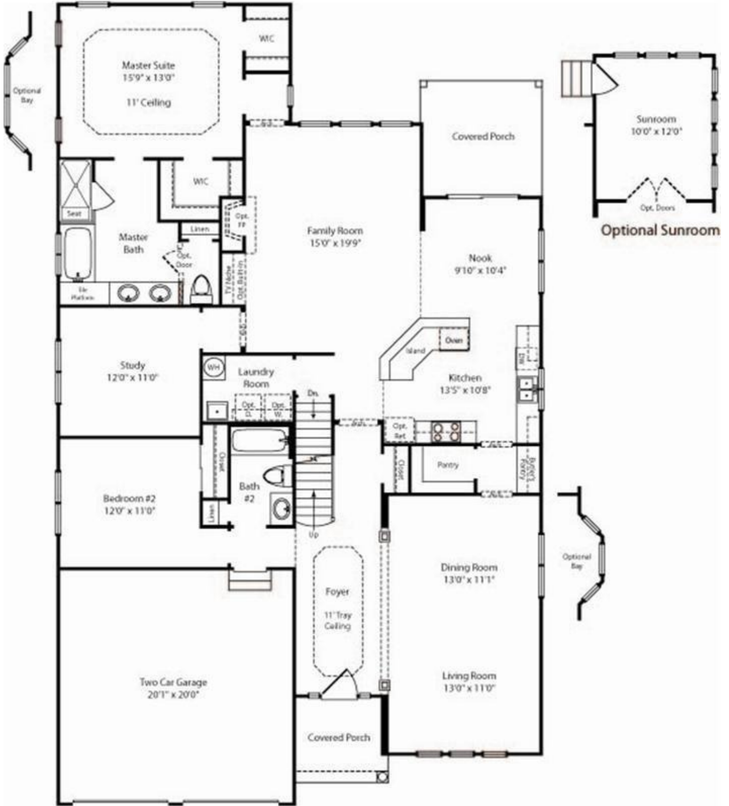
Donatello English Manor First Floor Plan
