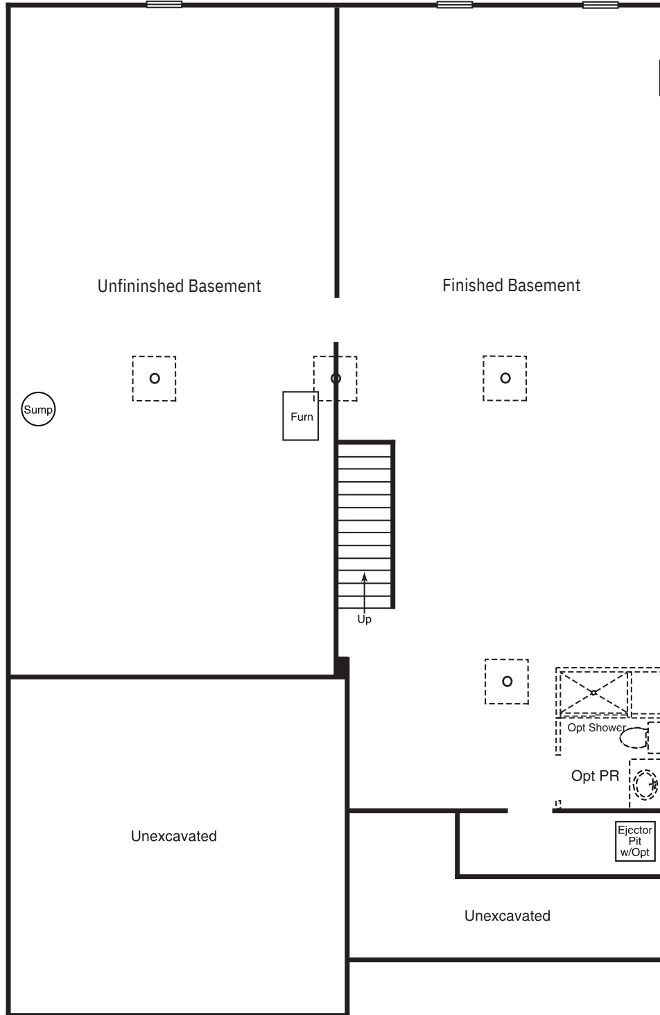
Optional Finished Basement Plan w/Optional Bath
