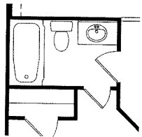
PARTIAL PLAN WITH 2ND DOOR TO BATH
