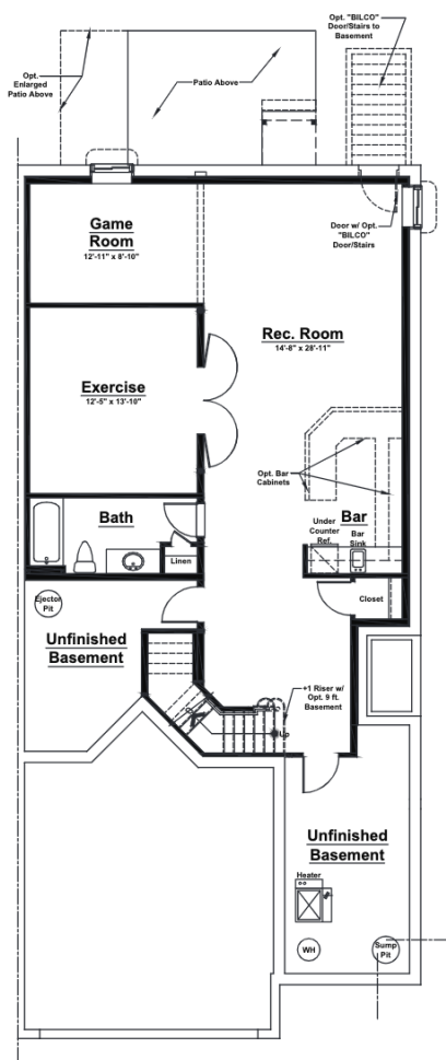
OPTIONAL FINISHED BASEMENT
