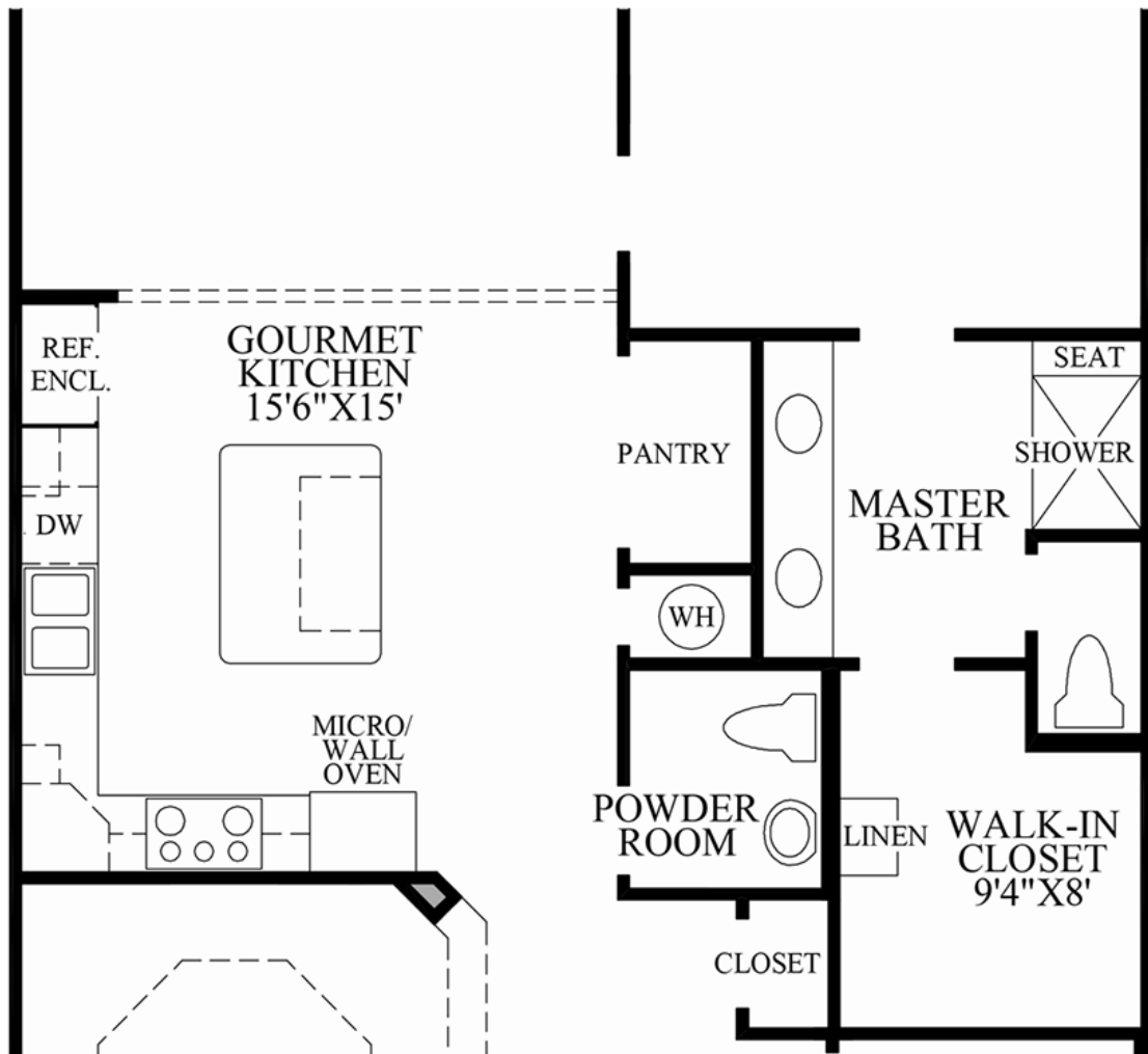
SHOWN WITH OPTIONAL ALTERNATE KITCHEN LAYOUT
